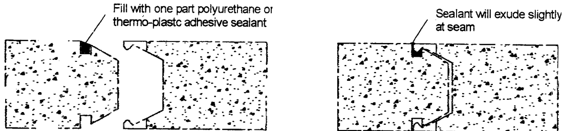
FIGURE 5 UNIVERSAL LOCKING
