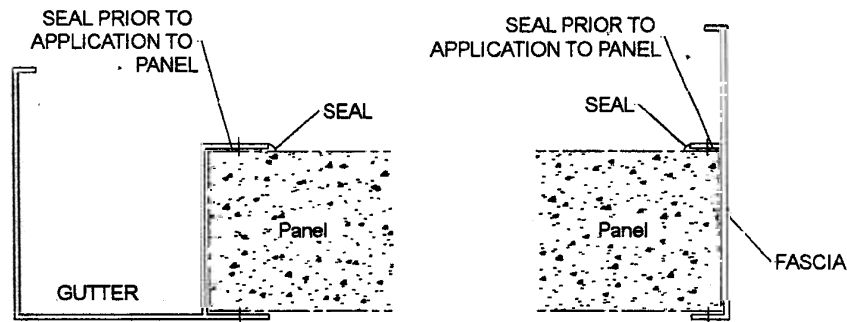
FIGURE 9 PANEL WITH GUTTER
