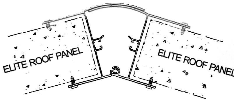
FIGURE 7 ELITE ADJUSTABLE RIDGE BEAM
