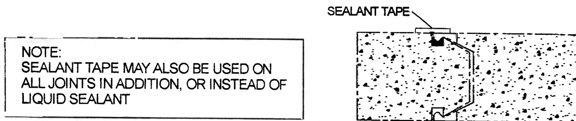
FIGURE 6 SEALANT TAPE
