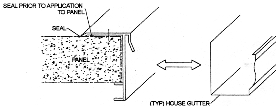
FIGURE 10 PANEL WITH DRIP-EDGE FASCIA
